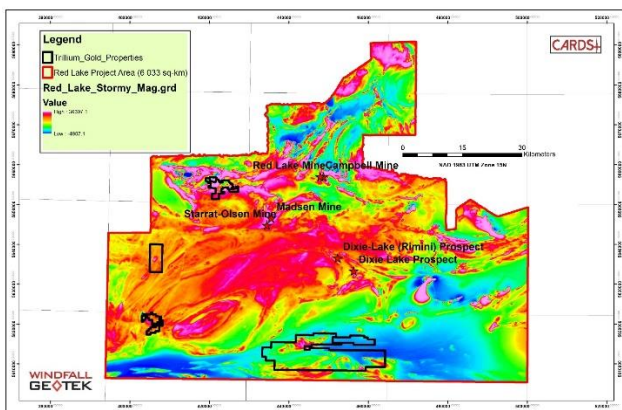
Figure 1: Regional gold signature based on the Ontario Supergrid Magnetic data (Red Lake-Stormy) and SRTM at 40m resolution
