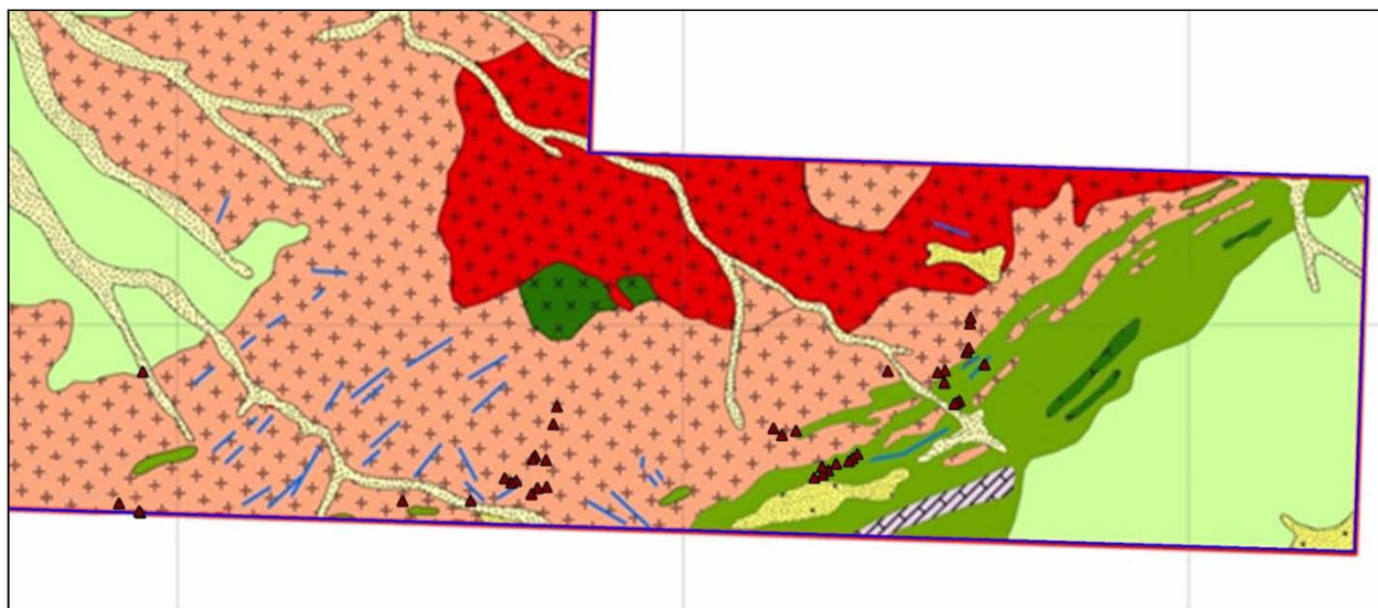
Figure 22. Locations of Rock Samples
