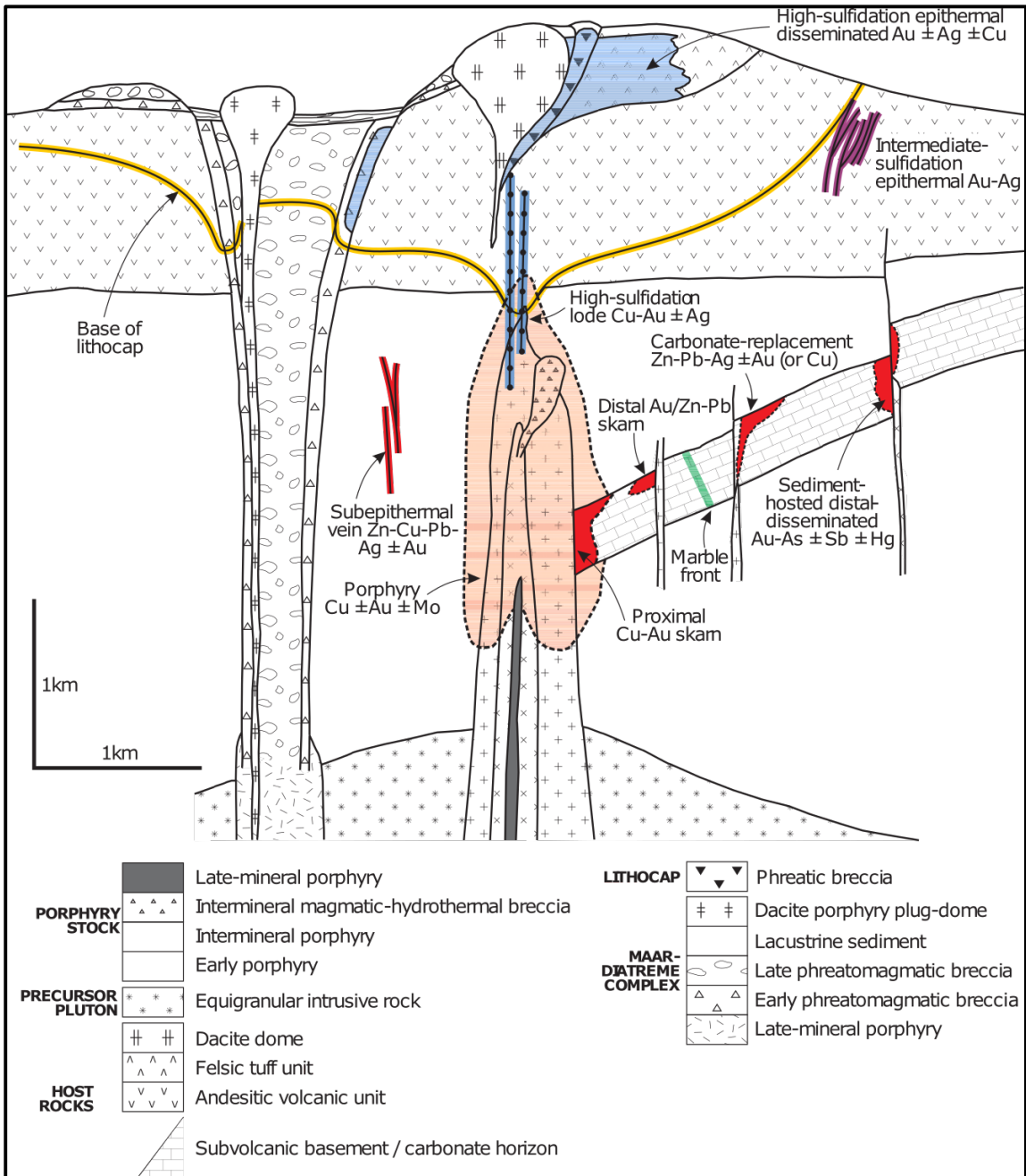
Figure 7: Deposit Model
