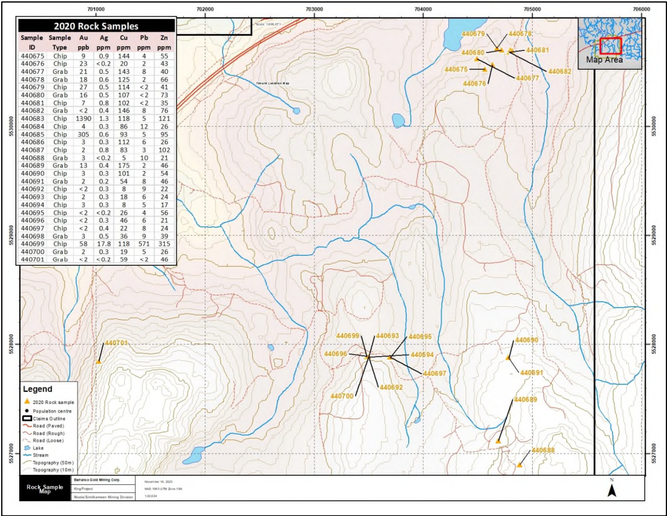
Figure 14: 2020 Rock Samples
