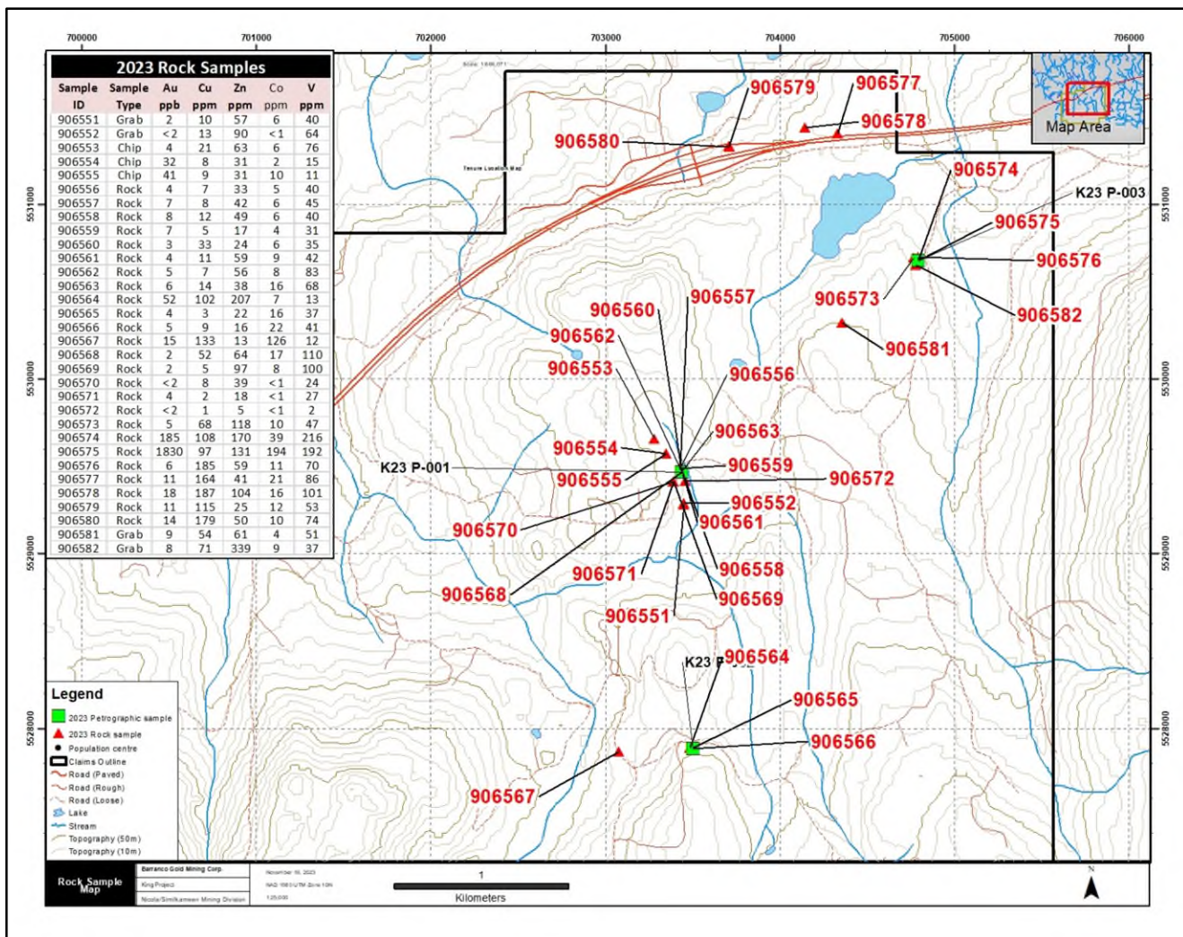
Figure 15: 2023 Rock Samples
