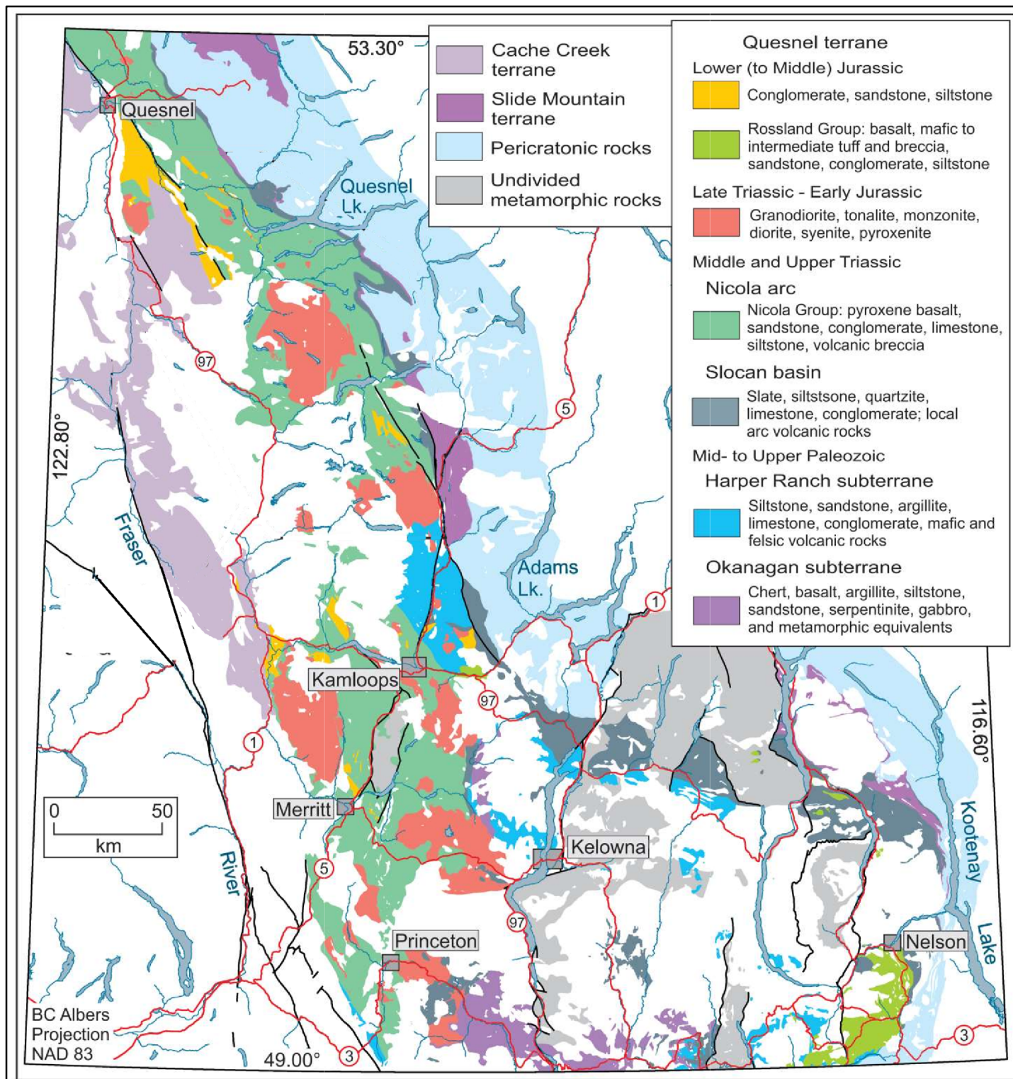
Figure 4: Regional Geology
