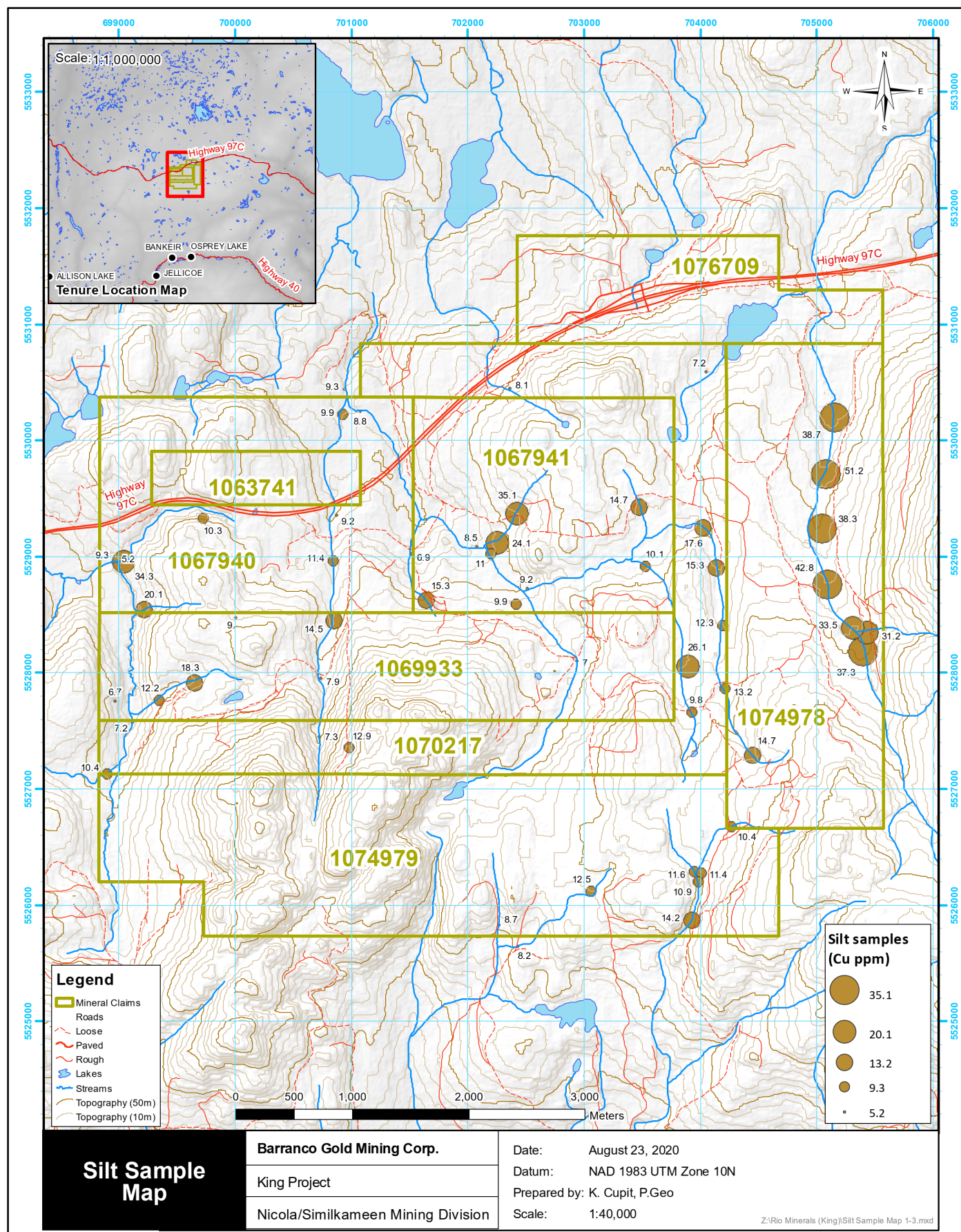
Figure 9: 2020 Copper in Streams
