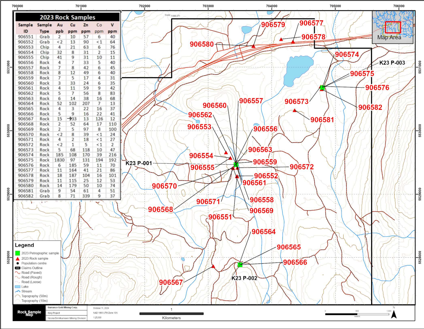
Figure 15: 2023 Rock Samples
