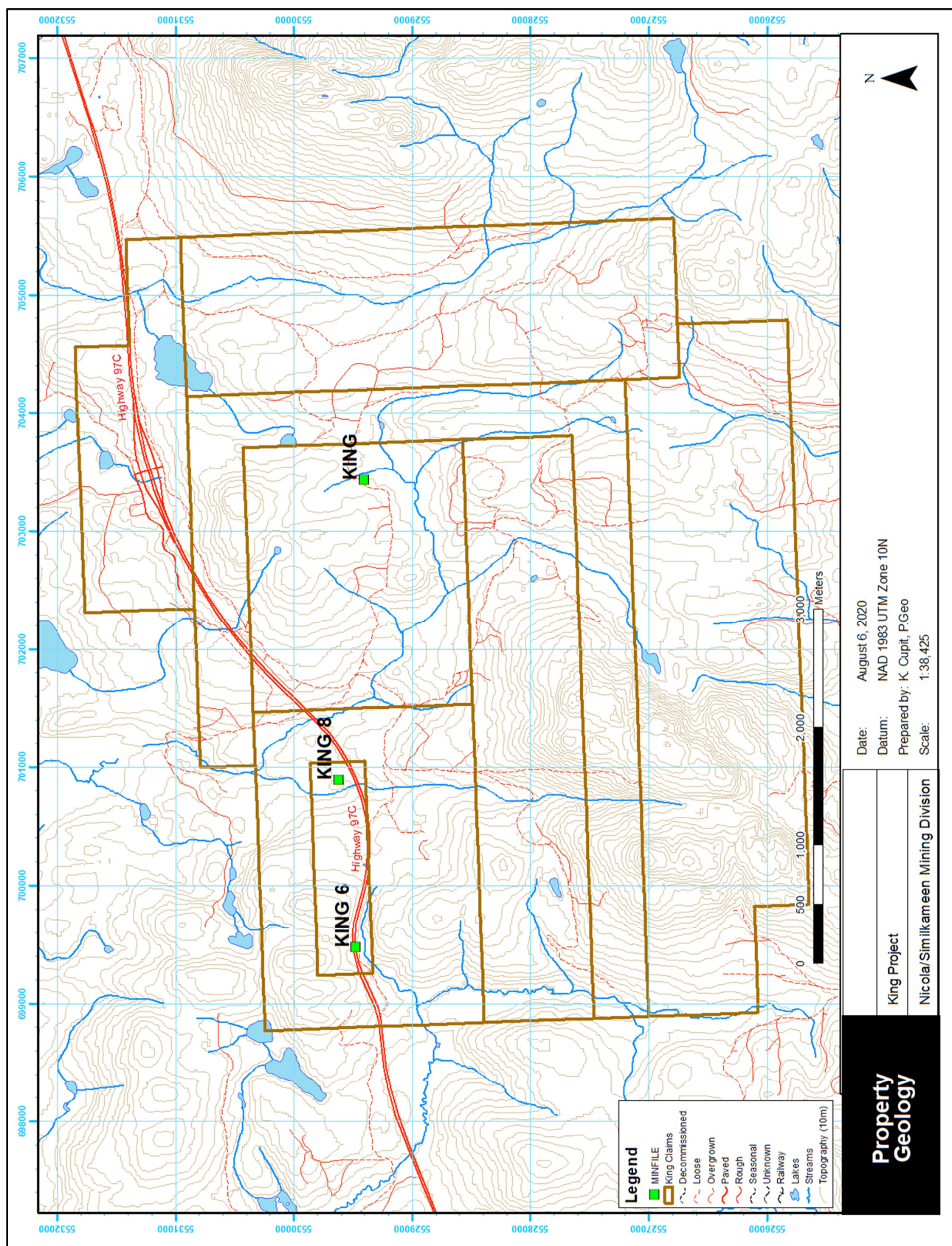
Figure 6: Minfile Showings
