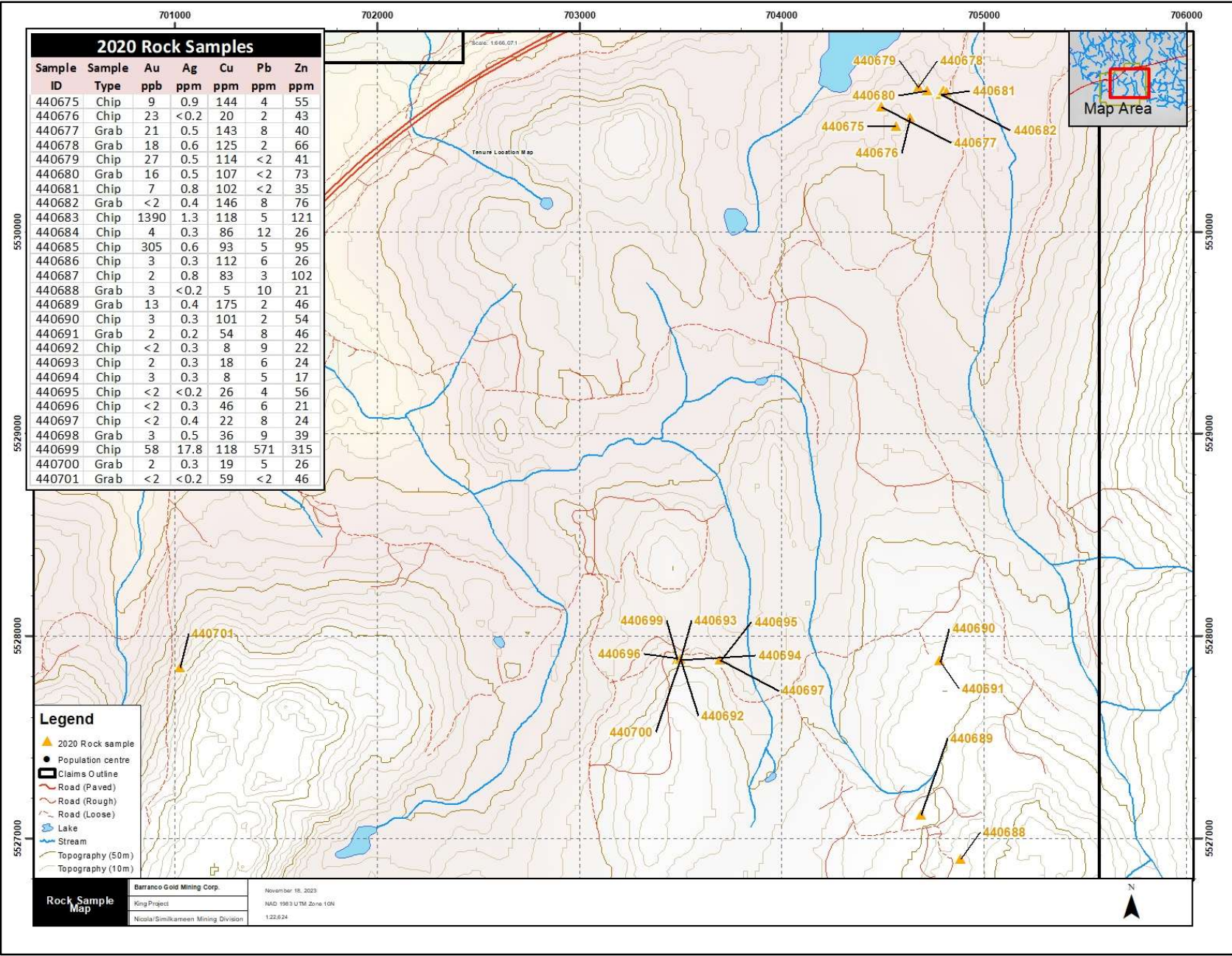
Figure 14: 2020 Rock Samples
