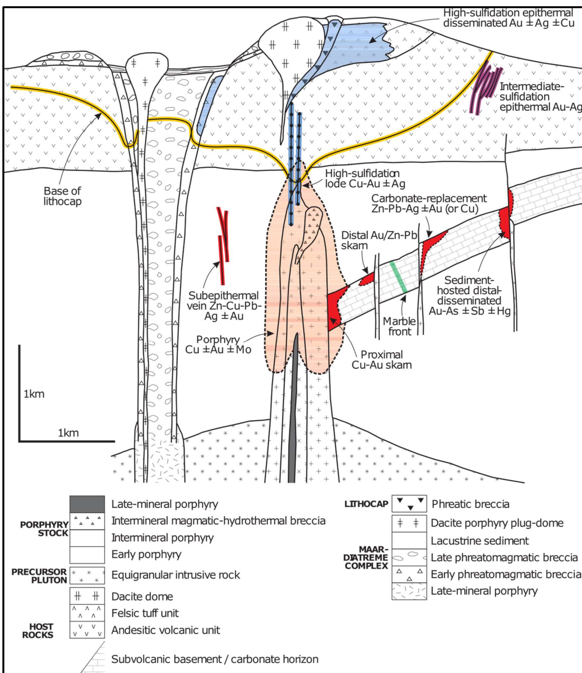
Figure 7: Deposit Model
