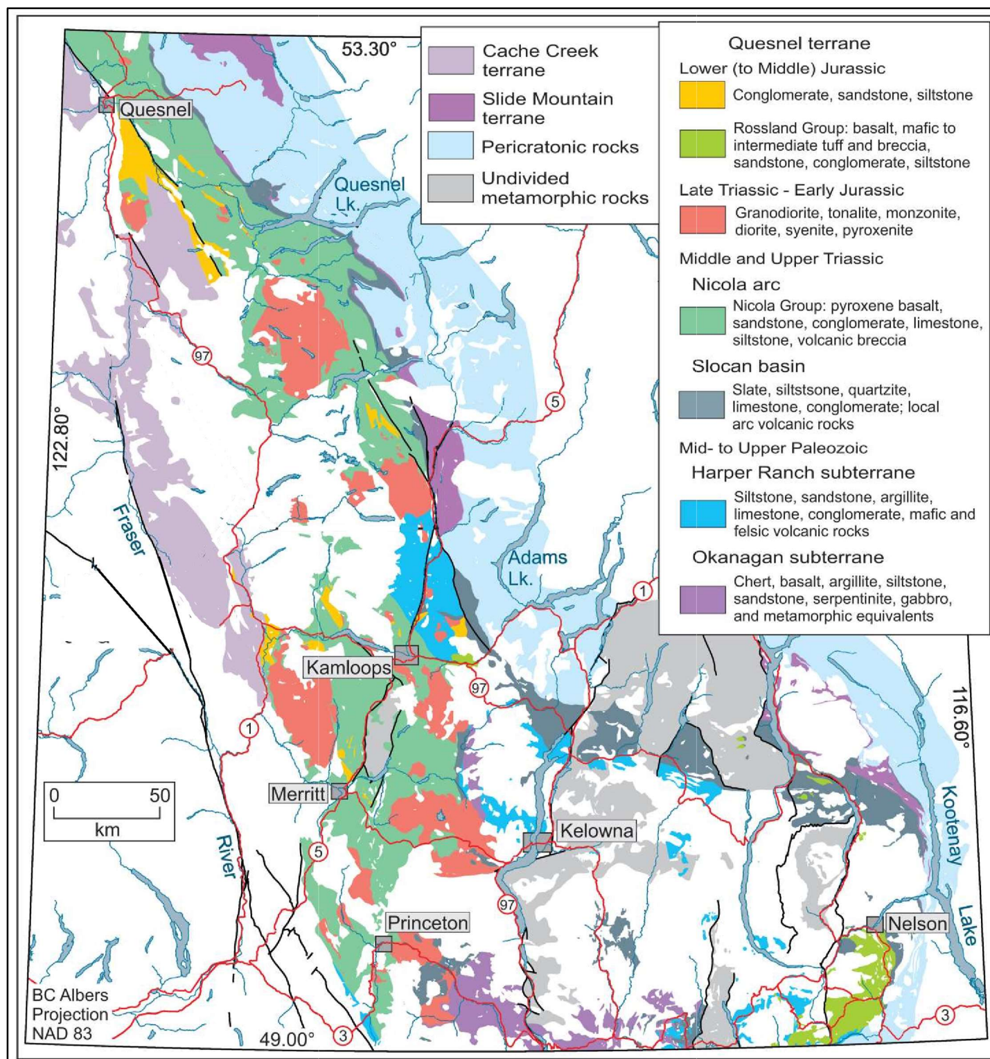
Figure 4: Regional Geology
