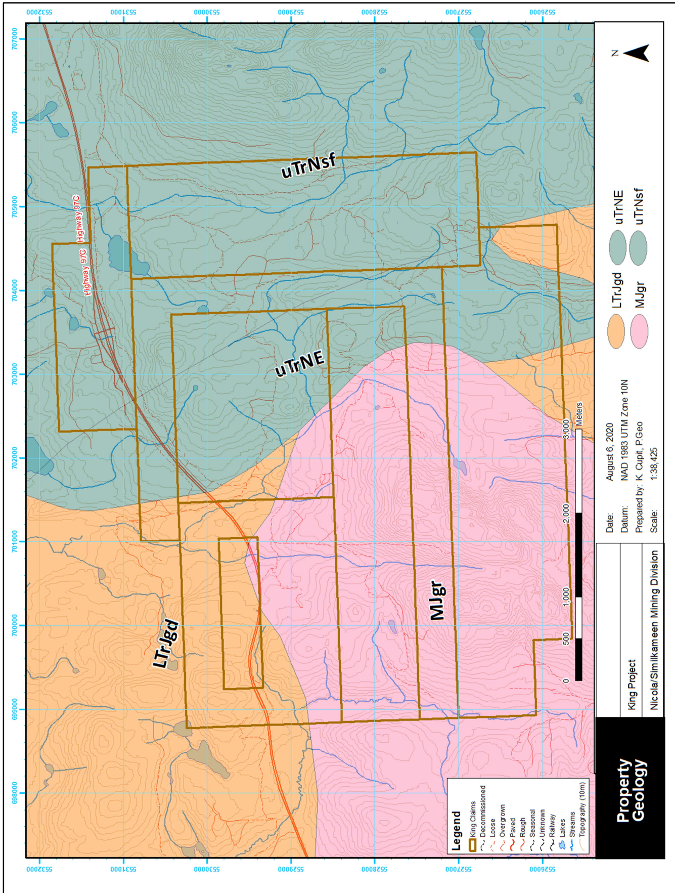
Figure 5: Property Geology
