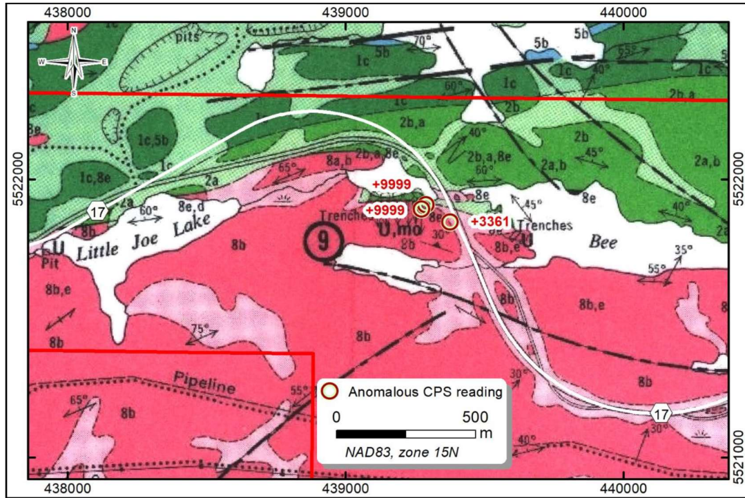
Figure 28: Bee Lake local geology showing the locations of the anomalous cps readings collected by R. Komarechka in an earlier site visit in 2020
