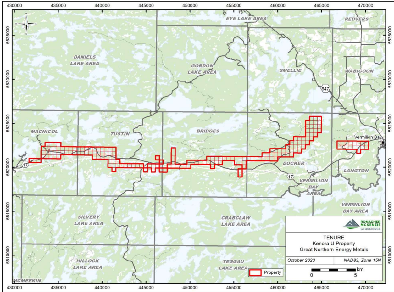
Figure 2: Claim fabric of the Kenora Property
