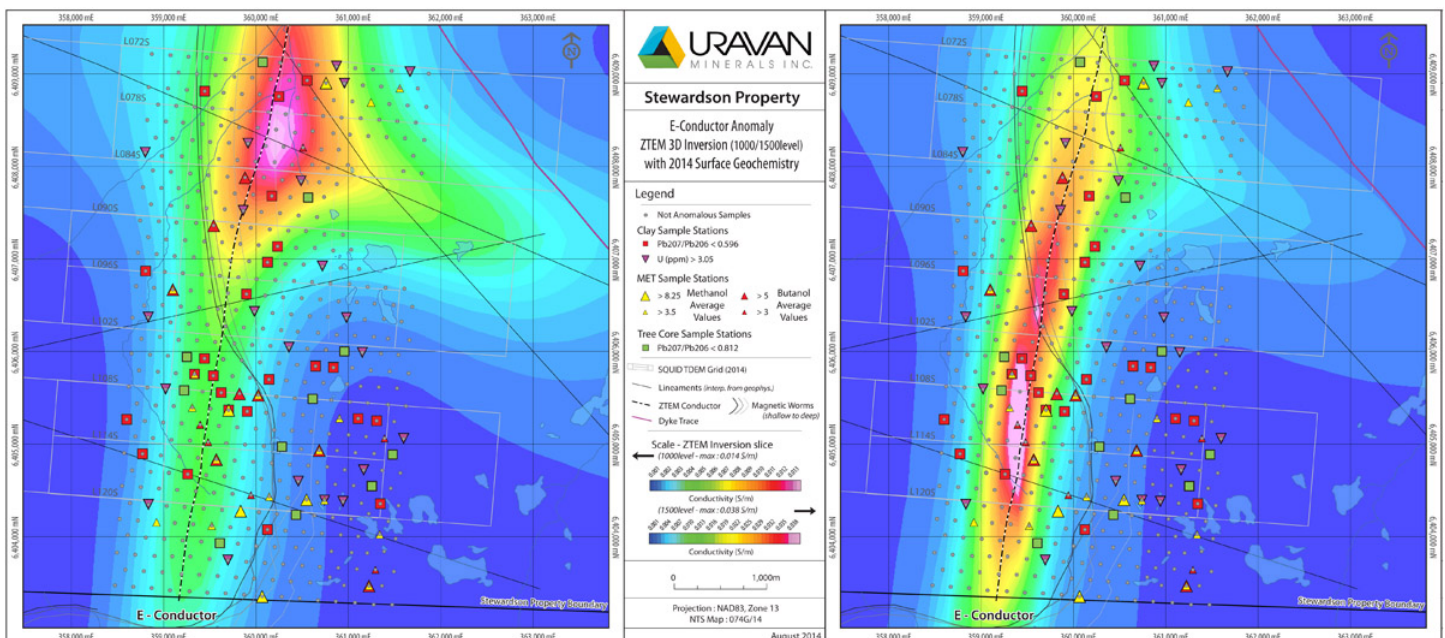
Figure 5 – E-Conductor (ZTEM 1000m and 1500m depth slice) with supported 2014 infill anomalous surface geochemistry and ground geophysical surveys.
