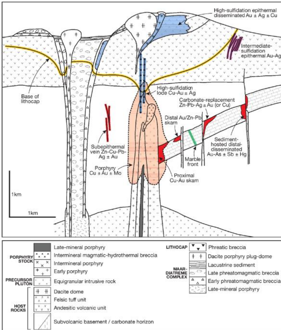
Figure 10: Deposit Model
