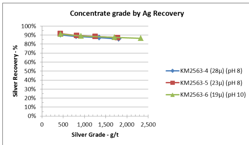
Figure 13-2: Cleaner Flotation Silver Performance
