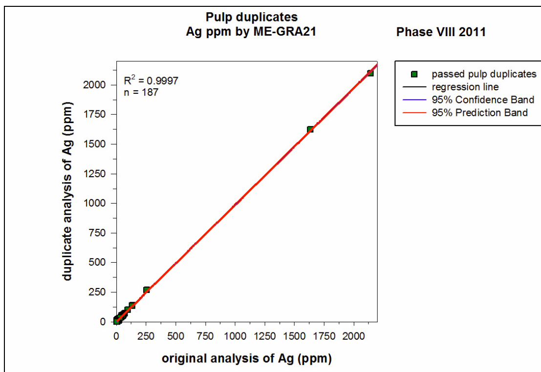
Figure 12-19: Pulp duplicate versus original plot for Ag analyzed with ME-GRA21 method
