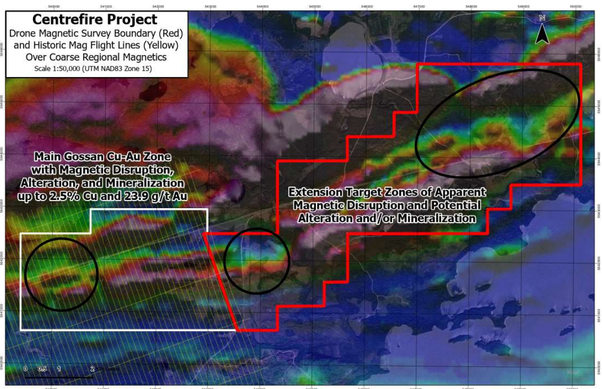
Figure 1: Area of Ongoing High-Resolution Drone Magnetic Surveying (Red) and Cu-Au Target Zones.
