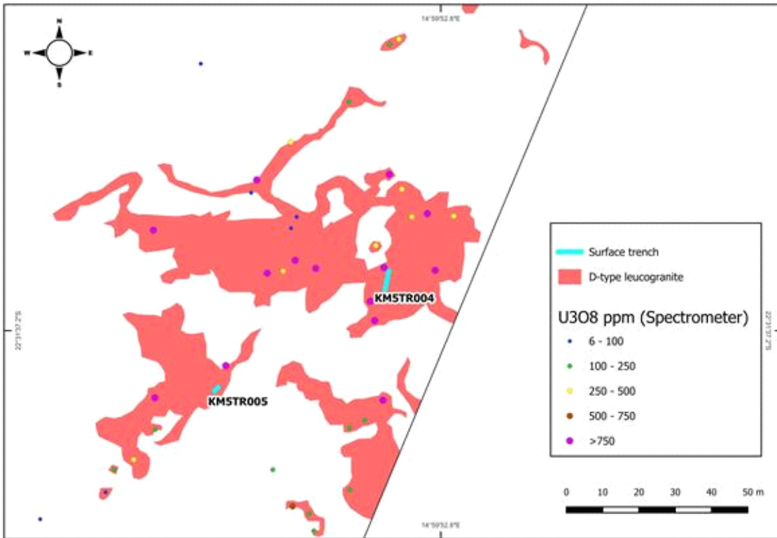
Figure 2: Mapped outcrop of D-type leucogranites in the vicinity of Trenches 4 and 5.
