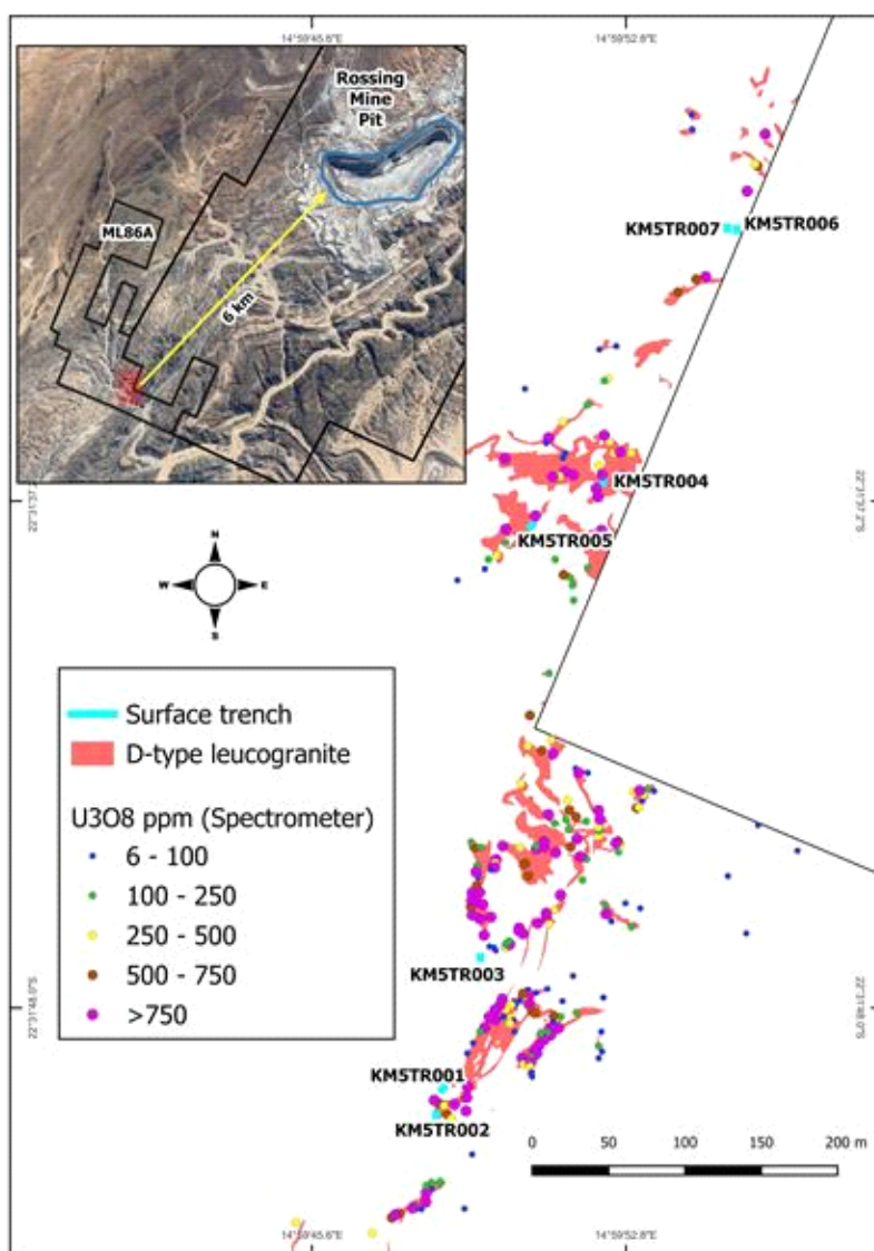
Figure 1: Location of Anomaly 5 and mapped D-type leucogranites at the Khan Project
