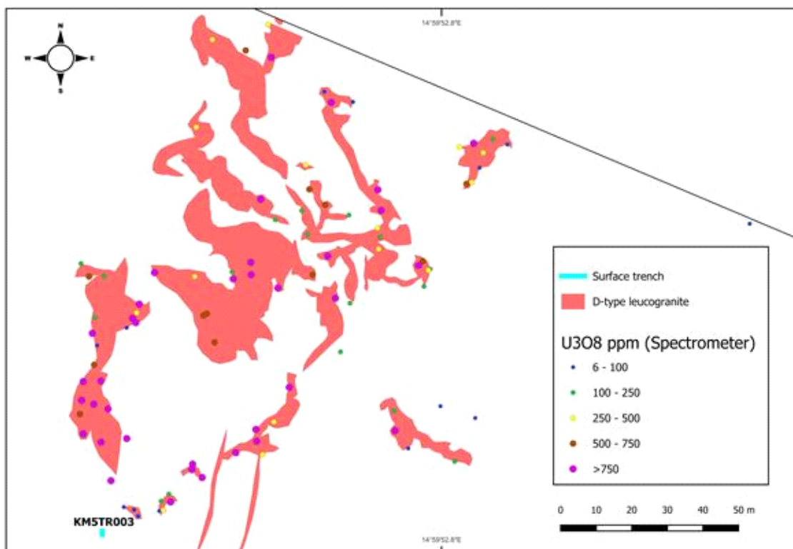
Figure 3: Mapped outcrop of D-type leucogranites north of Trench 3.
