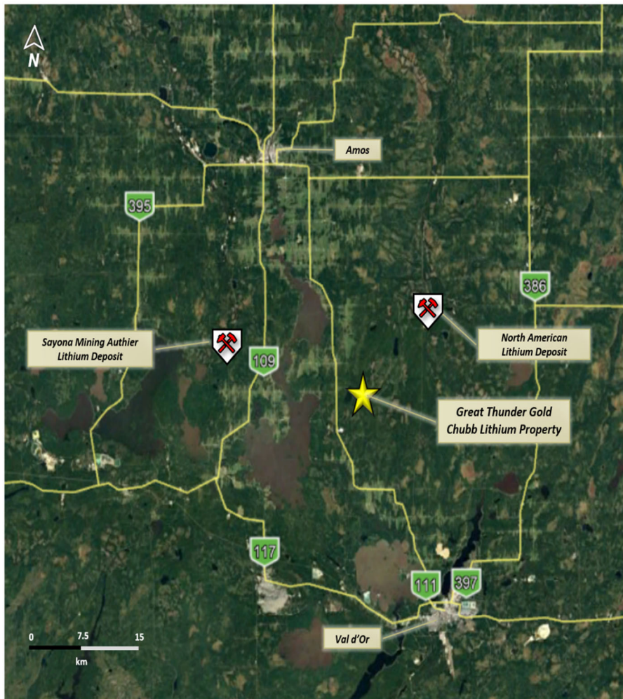
Figure 1: Regional location of the Chubb Property within the La Corne Pluton
