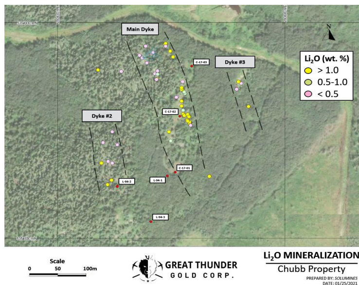
Figure 2: Pegmatite dyke swarm at the Chubb Lithium Property
