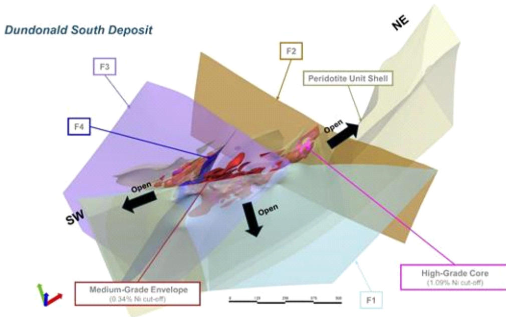
Figure 4. Isometric view of the D-S Deposit with 4 interpreted faults (F1 to F4) resulting in 3 primary target areas in which future drilling will aim to build additional mineralized high-grade nickel tonnes.
