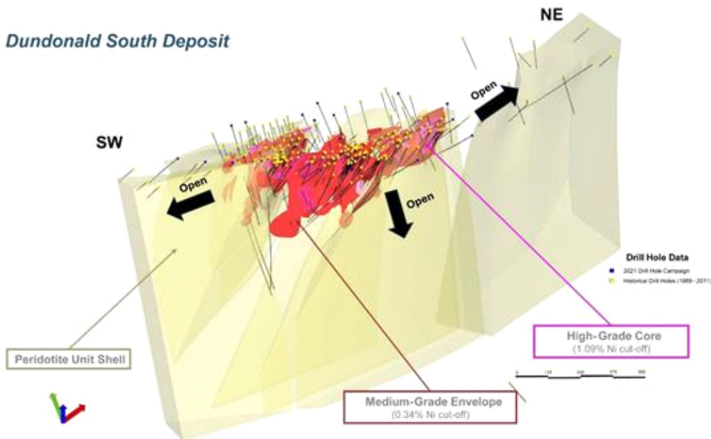
Figure 2. Newly interpreted 3D geological model (looking northwest) showing the high-grade nickel domain (core) and medium-grade nickel domain (envelope) that define the D-S Deposit, along with historical and Class 1 (2021) drill hole traces. The D-S deposit is open along strike and at depth.
