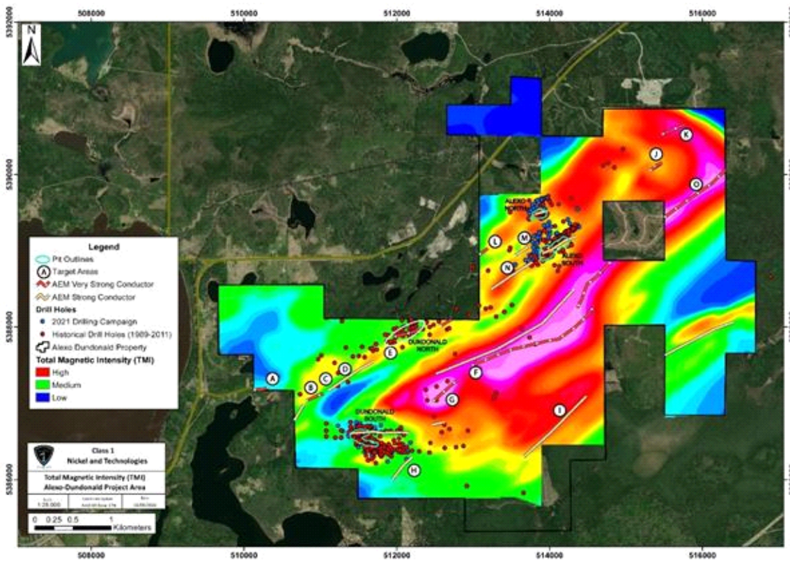
Figure 1. Alexo-Dundonald Nickel Project with regional Total Magnetic Intensity (TMI) and classified aero-electromagnetic (AEM) conductors from a 2020 VTEM survey. Locations of the 2024 Alexo South and Alexo North pit shells and the 2020 Dundonald South and Dundonald North pit shells (nickel deposits) are shown, along with historical drill hole collar locations.
