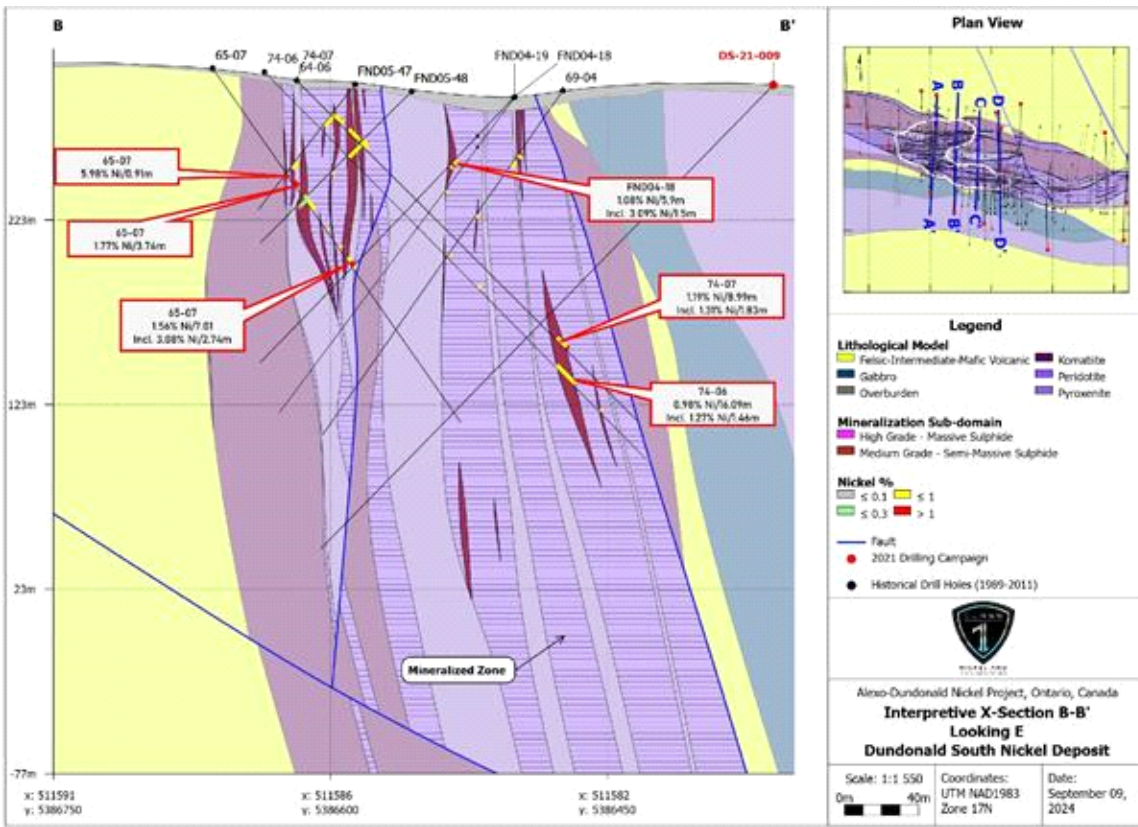
Figure 5. Cross-section (B-B' looking east) through the central Dundonald South Deposit showing the principal high-grade nickel zones. The newly modelled and interpreted geology, structures, and alteration provides numerous target areas for future drilling which will be aimed at building additional high-grade nickel tonnes. Reported intervals are not necessarily true widths and should be considered core lengths.
