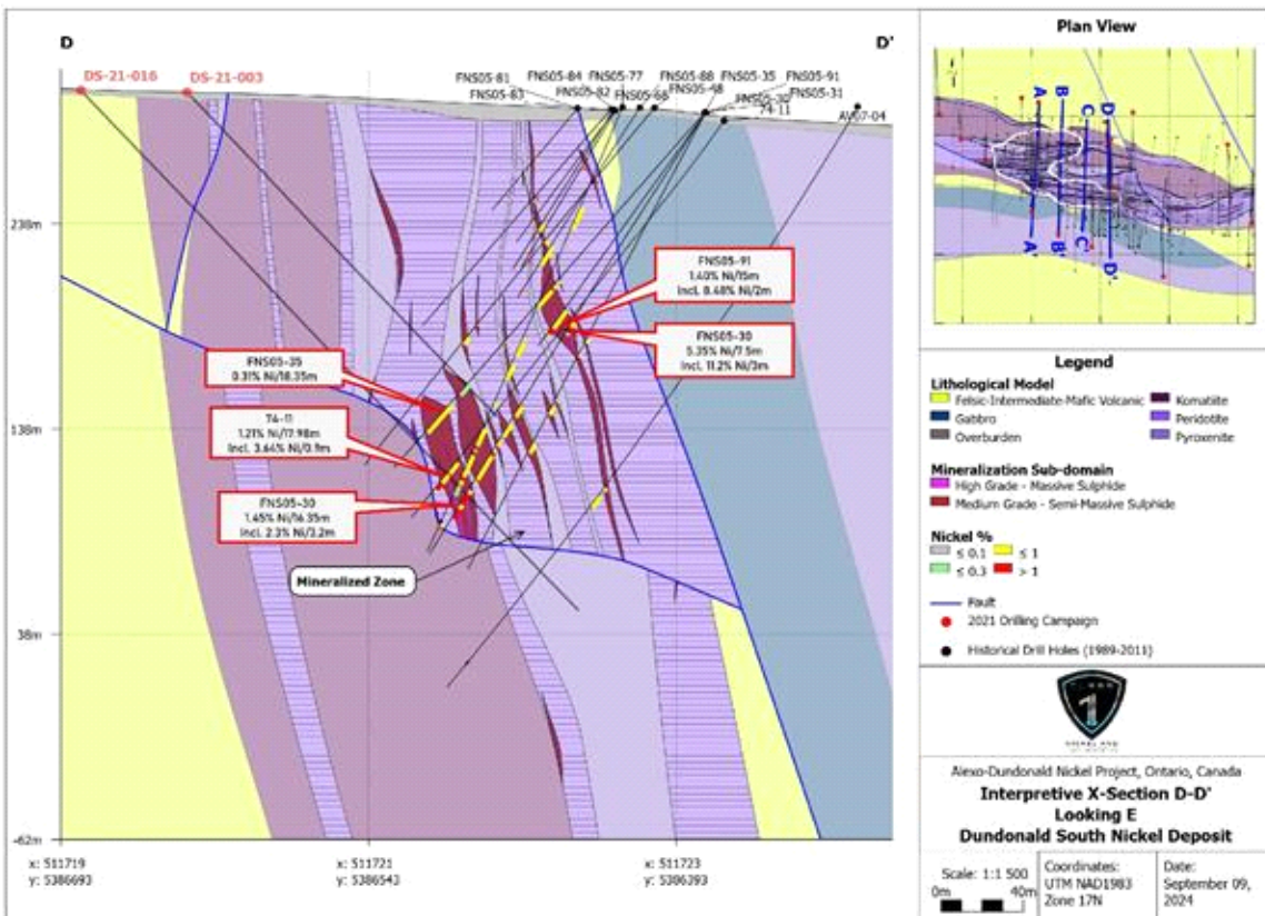
Figure 6. Cross-section (D-D' looking east) through the eastern Dundonald South Deposit showing the principal high-grade nickel zones. The newly modelled and interpreted geology, structures, and alteration provides numerous target areas for future drilling which will be aimed at building additional high-grade nickel tonnes. Reported intervals are not necessarily true widths and should be considered core lengths.
