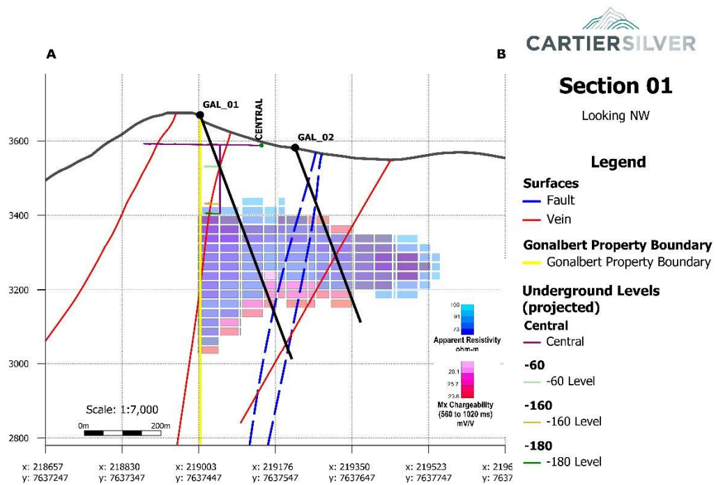
Figure 2: Cross Sections of Planned Drill Holes showing Location of Coincident Chargeability and Resistivity Anomalies being Drill-tested.
