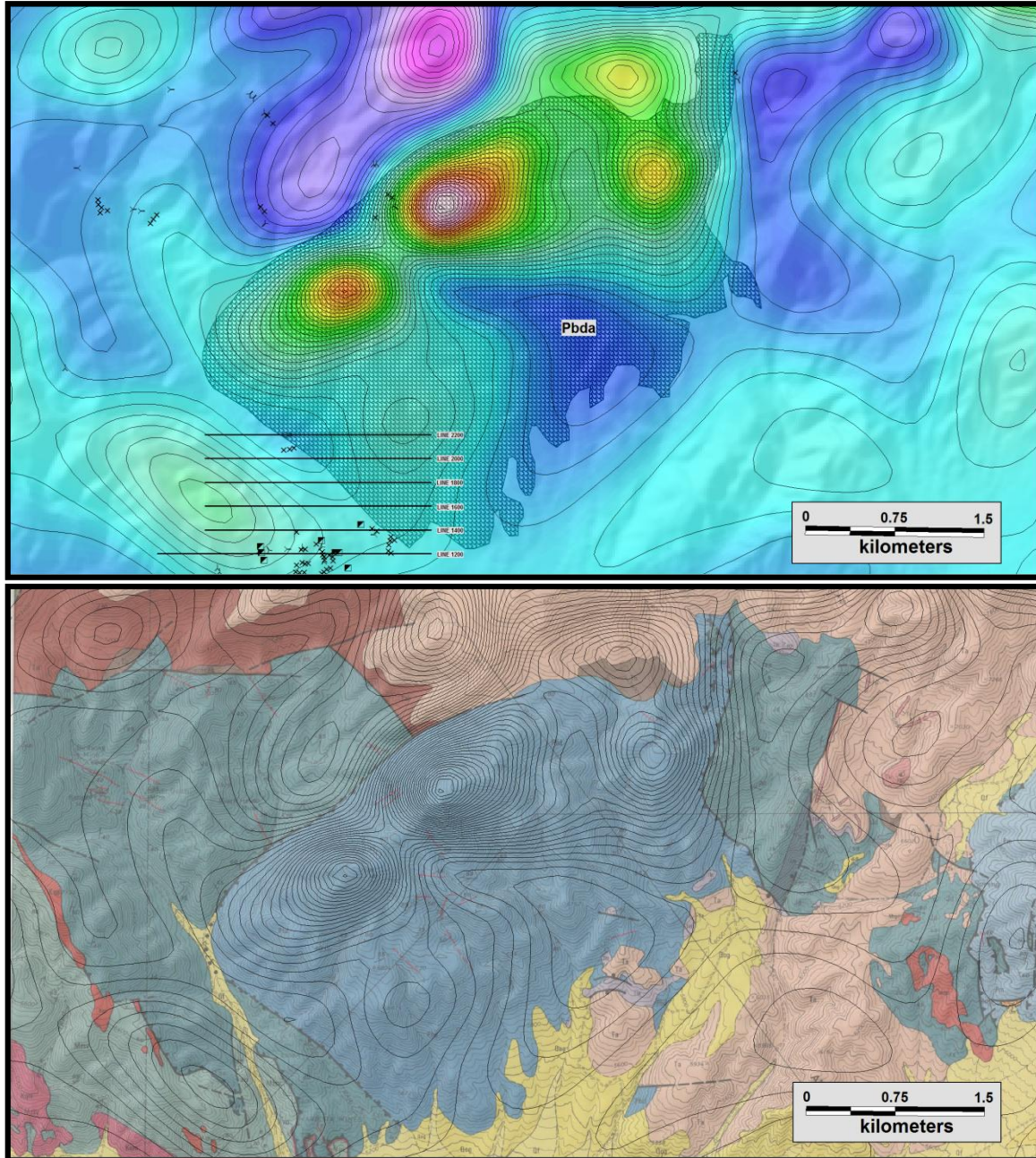
Figure 24: Airborne magnetics (USGS, 2001) and geology (Garside, 1982).
