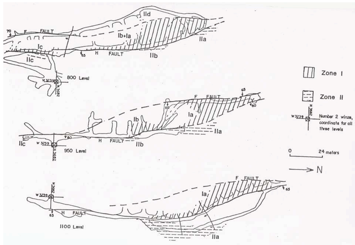
Figure 12: Clayton Silver Mine with mineralization in plan view for the north 800, 950 and 1100 levels (Hillman, Figure 14).
