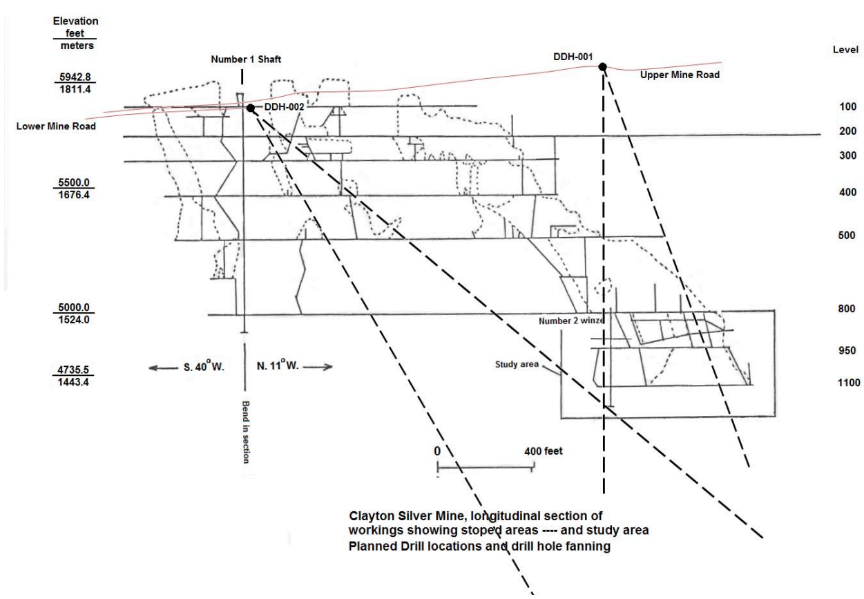
Figure 11: Clayton Silver Mine, longitudinal section of the underground workings showing stoped areas (dashed lines) and Hillman (1986) study area. (Hillman, Figure 6). The locations of proposed drill locations are also shown.
