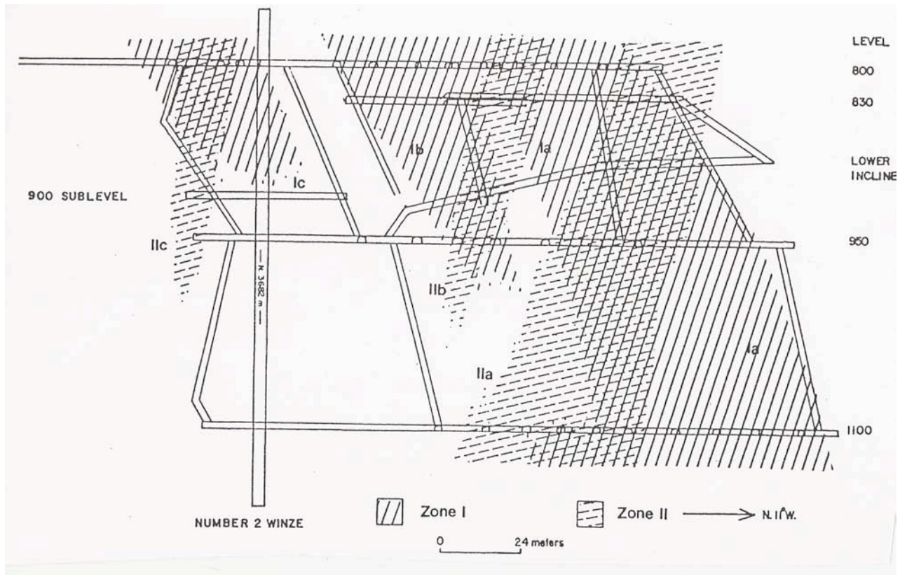
Figure 13: Clayton Silver Mine longitudinal showing ore shoots projected to the hanging wall fault (Hillman, Figure 15 – see his text for details).
