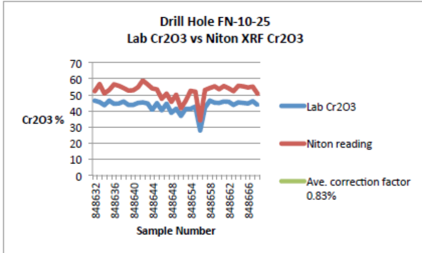
Figure 24.1 - Comparison of Niton XRF readings, prior to application of correction factor, and Lab Results for hole FN-10-25 (Armstrong, 2013).
