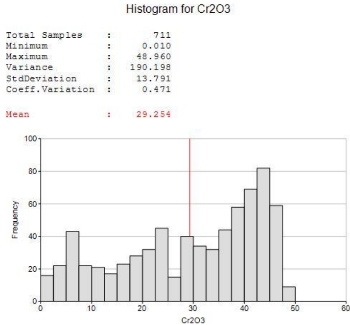
Figure 14.3 - Histogram of Cr 2 O 3 for Koper Lake Project.
