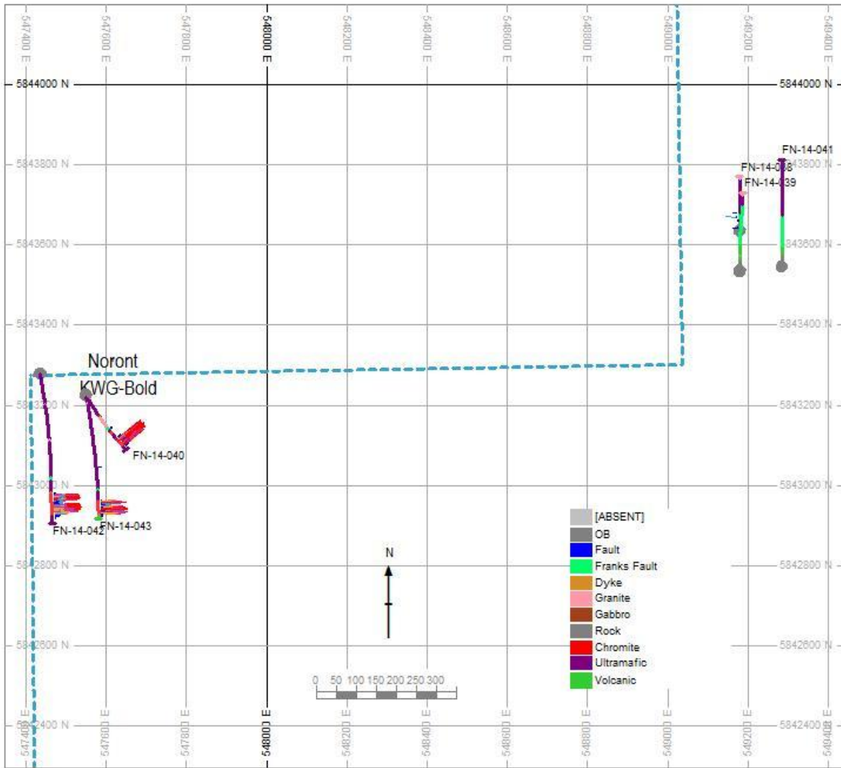
Figure 7.3 – Plan showing the six holes drilled in 2014.
