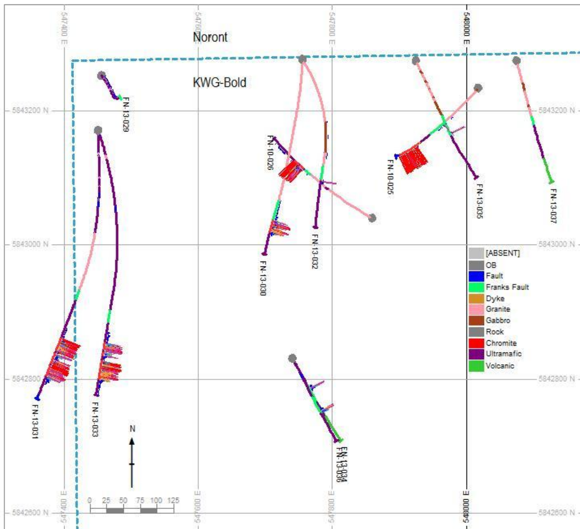
Figure 7.2 – Plan showing the Black Horse discovery holes (FN-10-025 and 026) and the nine holes drilled in 2013.
