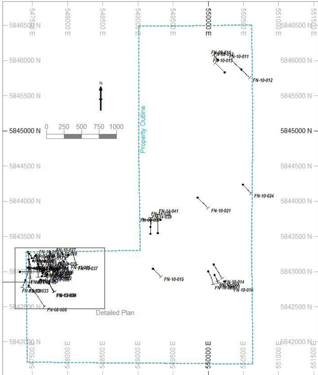
Figure 10.1 - Plan of Koper Lake Project Diamond Drilling.
