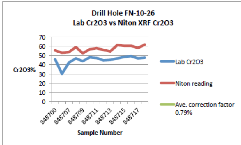
Figure 24.2 - Comparison of Niton XRF readings, prior to application of correction factor, and Lab Results for hole FN-10-26 (Armstrong, 2013).
