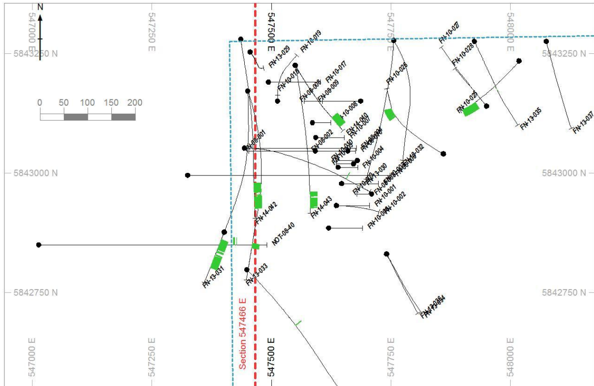
Figure 10.2 - Detailed Plan of Koper Lake Project Diamond Drilling showing location of example section 547466 E. Green bars are chromite intersections.
