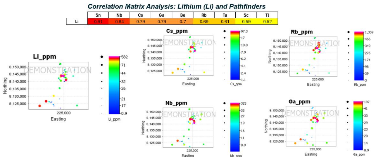
Figure 2: Lithium and pathfinder elements correlation and variable maps
