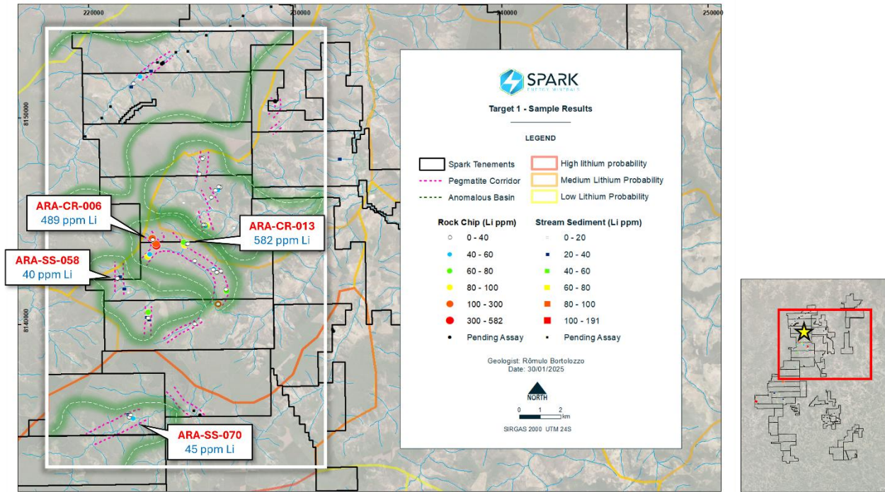
Figure 3: Target 1 showing location of mapped pegmatite trend now confirmed by positive lithium analytical results
