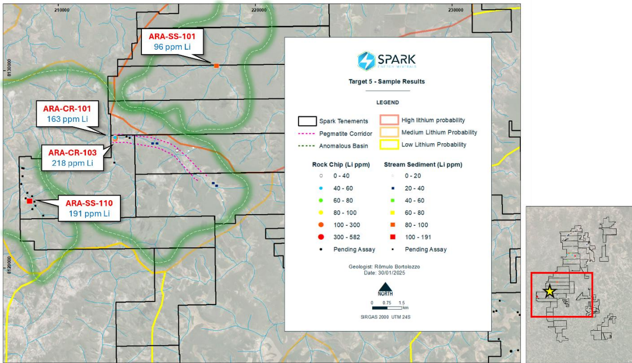
Figure 4: Target 5 showing location of mapped pegmatite trend now confirmed by positive lithium analytical results
