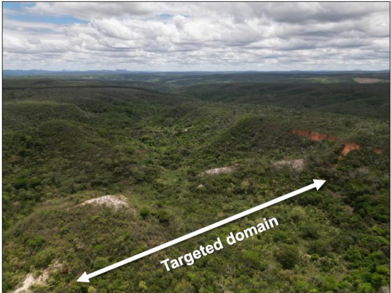
Figure 2: Drone view targeted trending domain within an erosional window beneath the overburden as seen in red/orange exposure on the right-hand side
