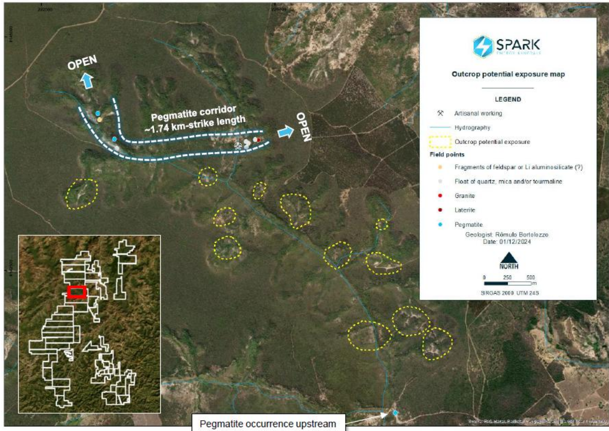
Figure 1: Mapped pegmatite corridor trending east-west spanning 1.74km in the northern half of the Arapaima Lithium project tenements
