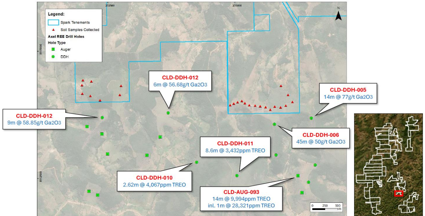
Figure 4: Figure showing recent TREO and Gallium – Ga203 results reported by Axel exploration, (green dots show drill holes with red dots depicting soil samples collected by Spark immediately to the north of the Spark – Axel tenement boundary.
