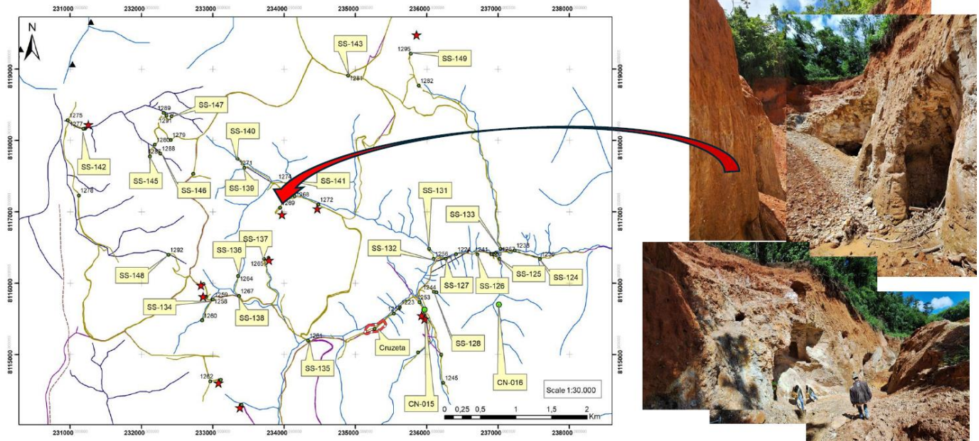
Figure 2: Integrated Map with stream sediment sampling stations and old mining excavations
