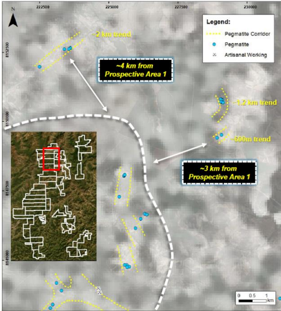
Figure 1: New Pegmatite Trends Northeast and Northwest of Target Area 1. These trends add 3.8km of pegmatite strike increasing the current target inventory to 31km.
