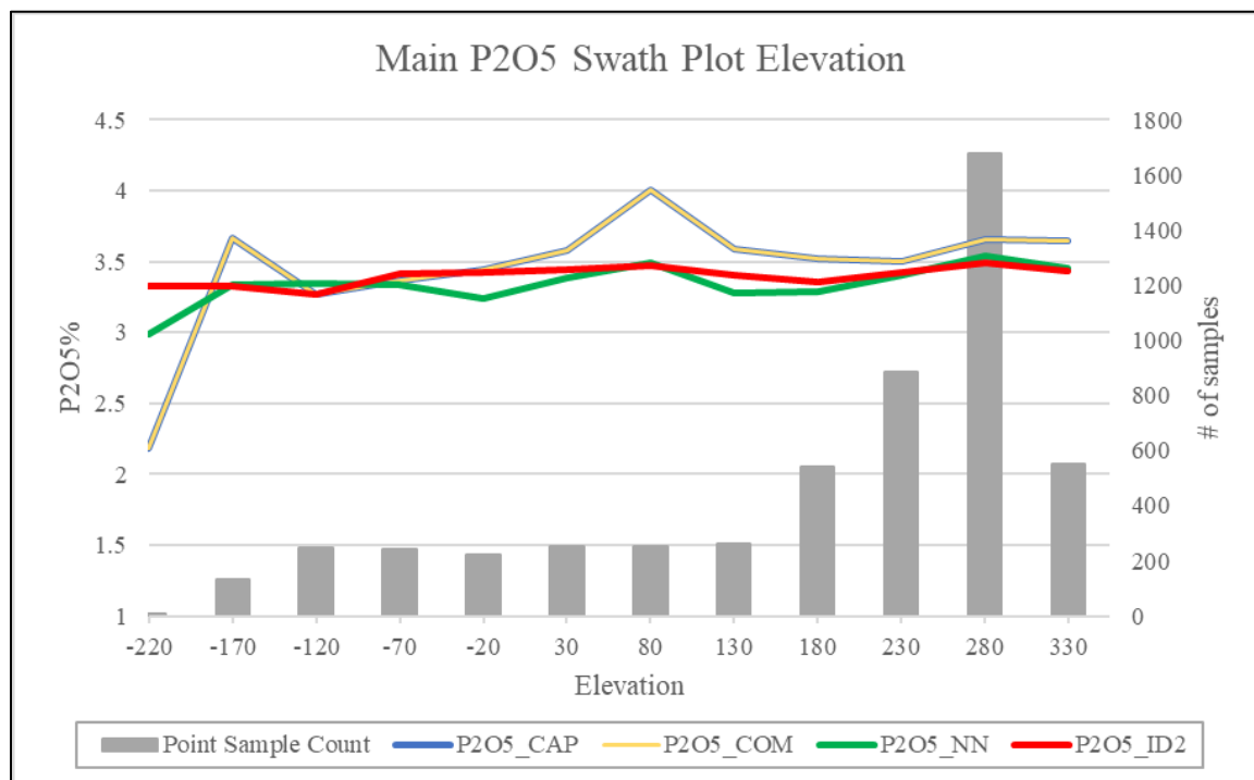
FIGURE 14.4 MAIN DOMAIN P 2 O 5 GRADE SWATH ELEVATION PLOT
