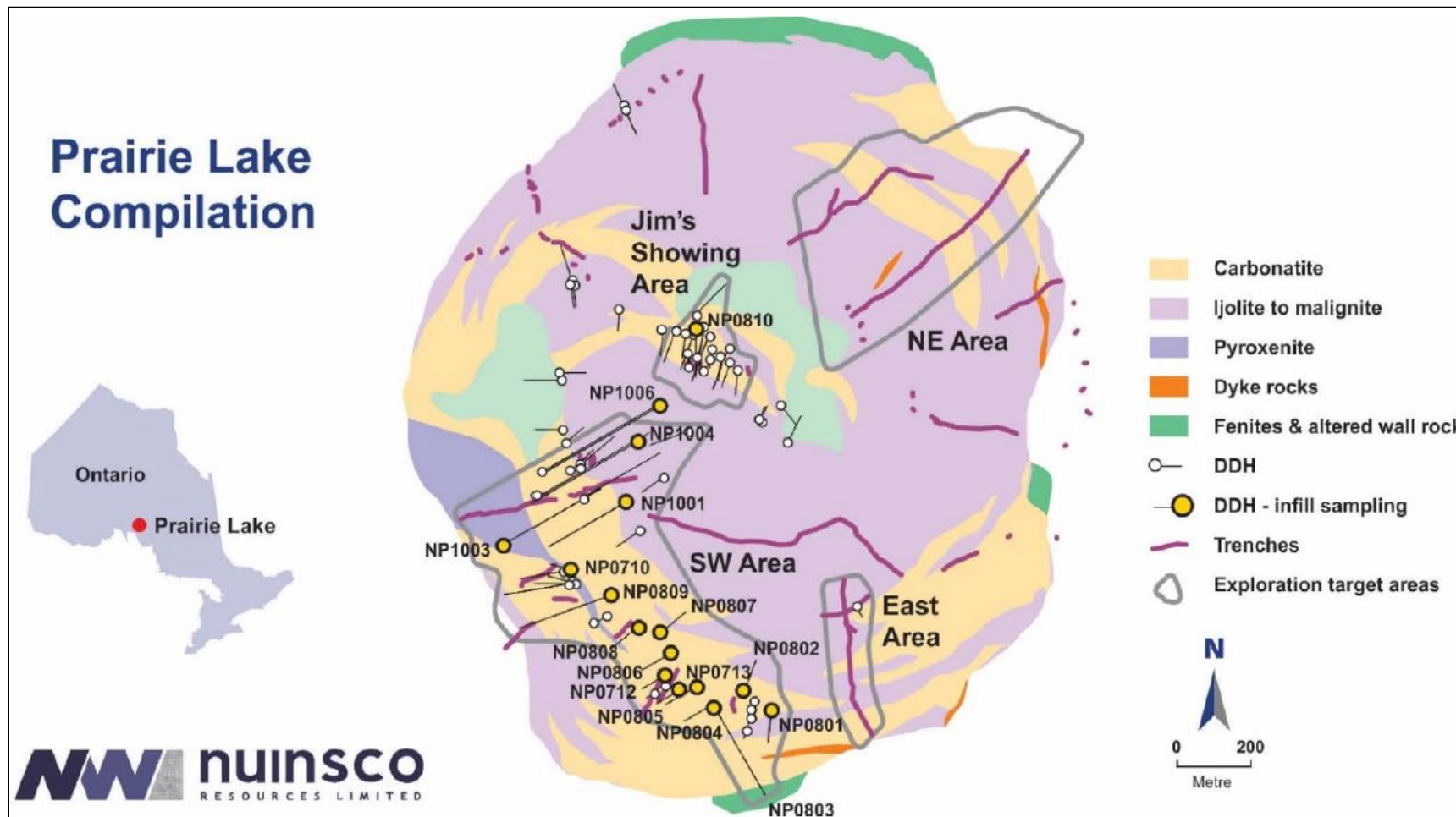
FIGURE 6.1 PLCC TARGET AREA LOCATIONS
