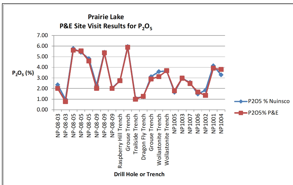
FIGURE 12.4 P&E SITE VISIT RESULTS FOR P 2 O 5
