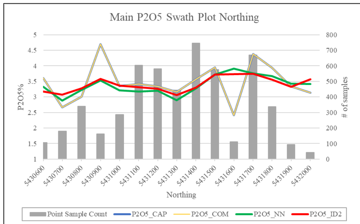
FIGURE 14.3 MAIN DOMAIN P 2 O 5 GRADE SWATH NORTHING PLOT
