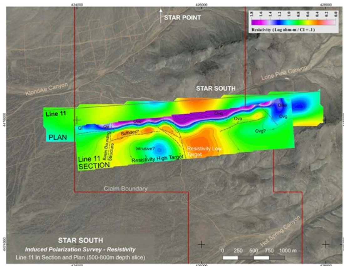
Figure Line 11: Star South IP Resistivity Inversion showing Section and Plan (500-800m depth slice)
