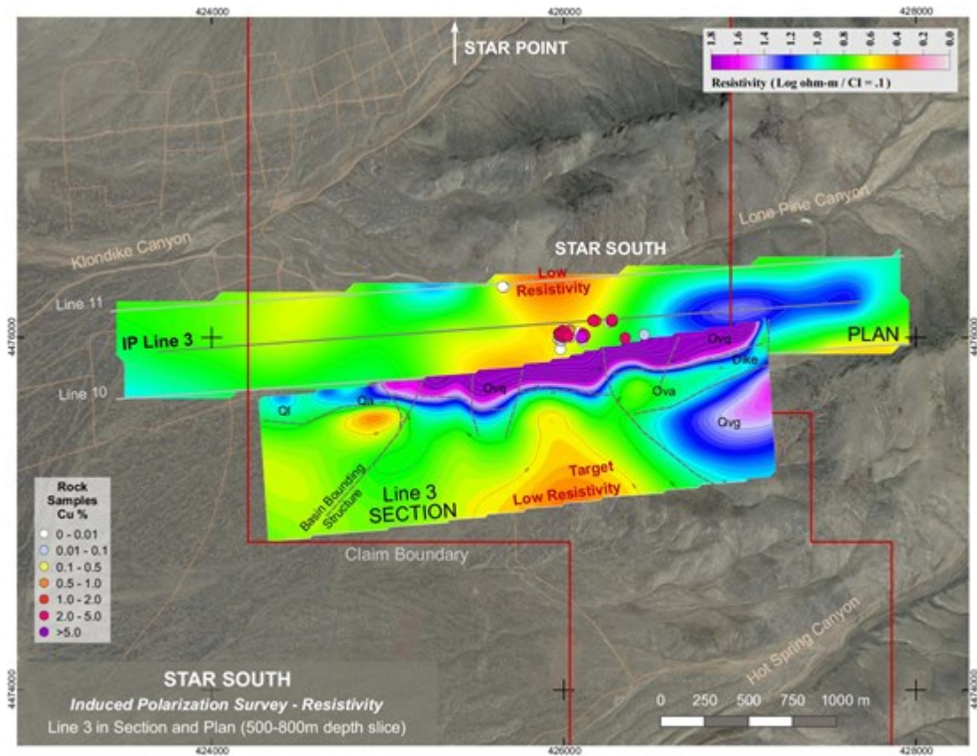
Figure Line 3: Star South IP Resistivity Inversion showing Section and Plan (500-800m depth slice)
