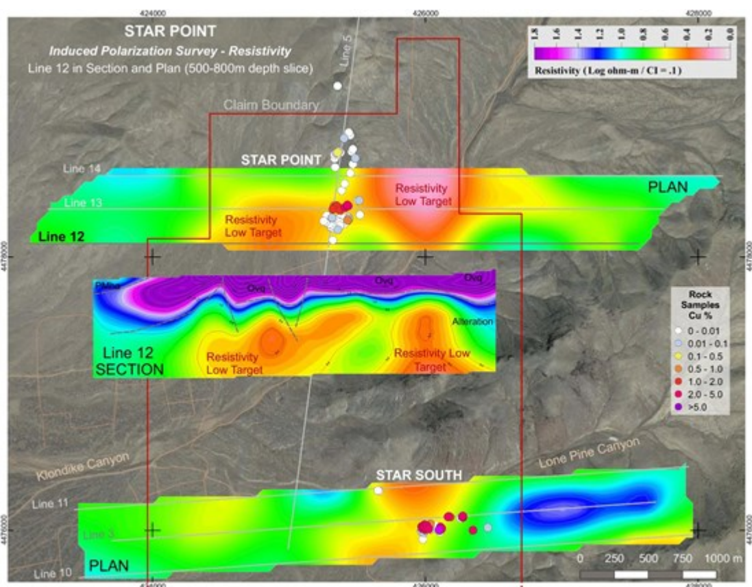
Figure Line 12: Star Point IP Resistivity Inversion showing Section and Plan (500-800m depth slice)
