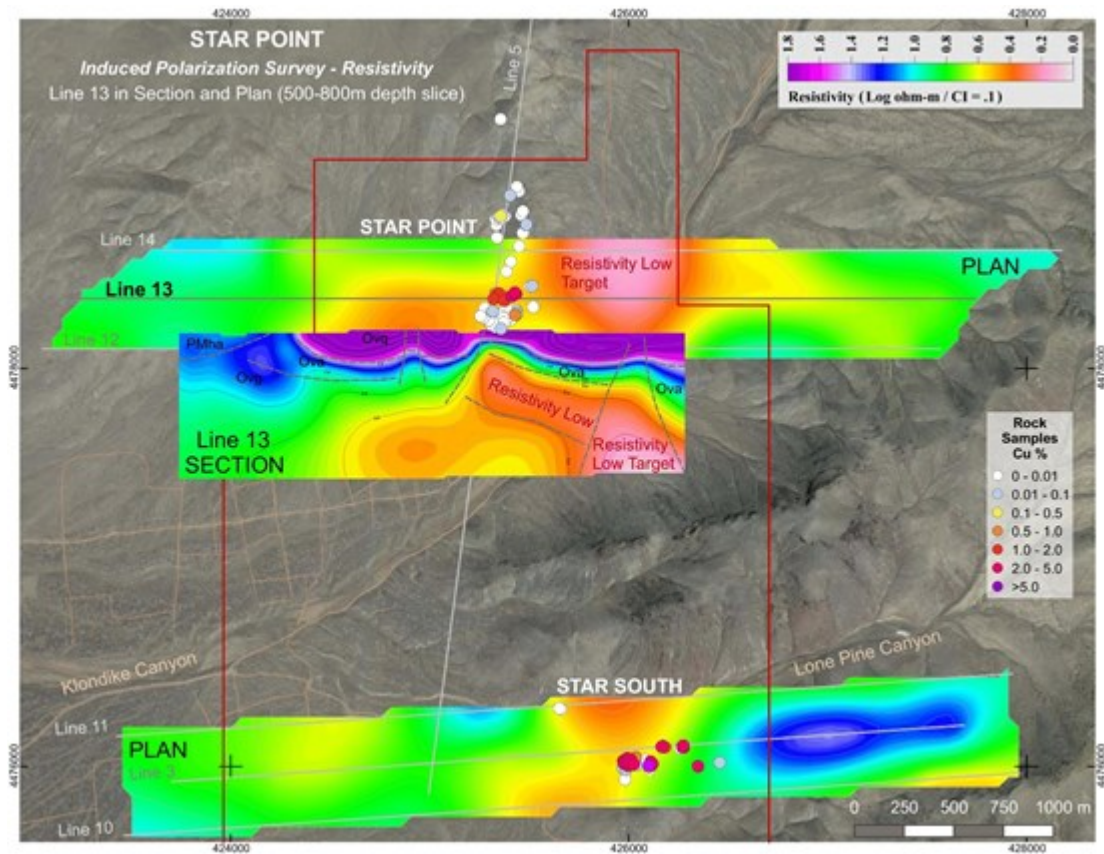
Figure Line 13: Star Point IP Resistivity Inversion showing Section and Plan (500-800m depth slice)
