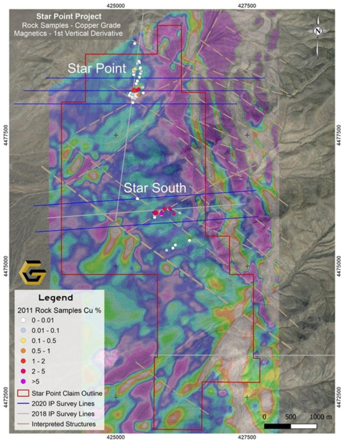
Figure 2: Star Point project area showing 2011 rock grab sample copper results, 2018 and 2020 IP survey lines and 2018 magnetic survey 1 st vertical derivative.
